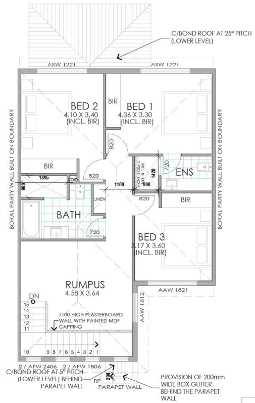
FLOOR PLAN - UPPER SCALE 1:100 @ A3
