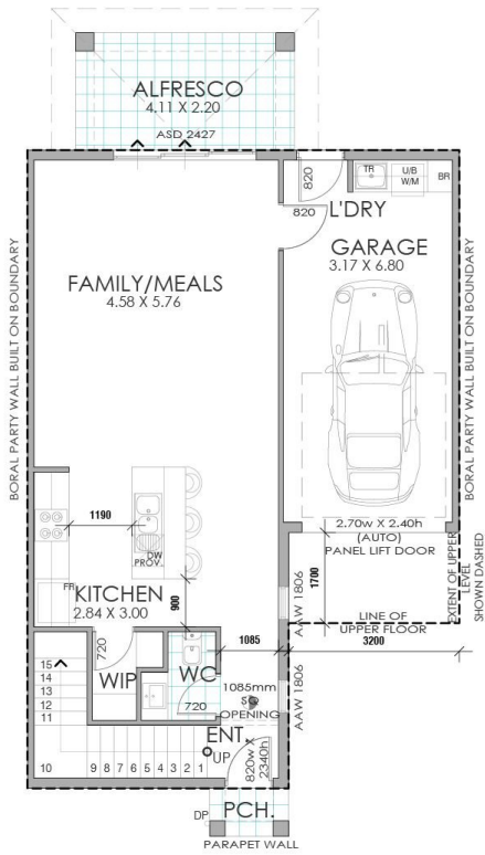
FLOOR PLAN - GROUND SCALE 1:100 @ A3
